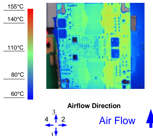
Figure 8. Thermal Image for Airflow Direction 3 (39A output, 55°C ambient, 200 LFM, typical Vin, open frame unit)
